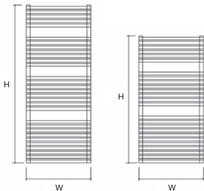
H150 - 30 tubes
